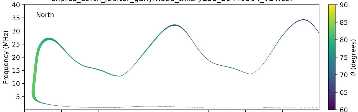
expres_earth_jupiter_ganymede_txka-y235_20440504_v14.cdf
