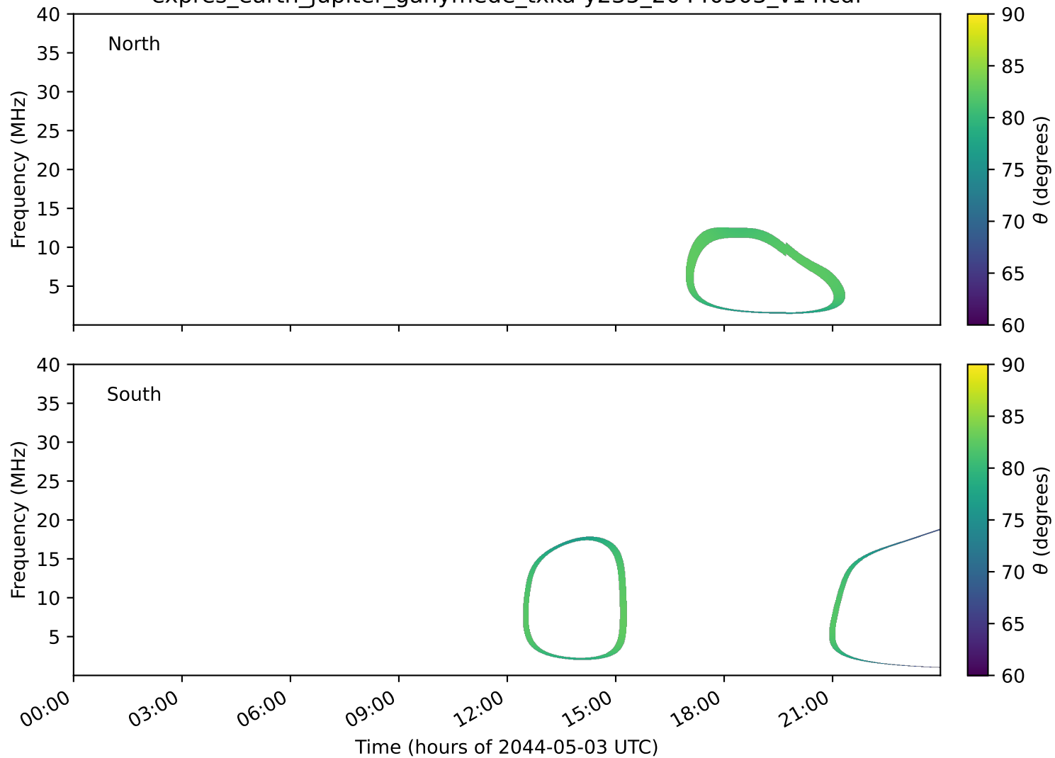
expres_earth_jupiter_ganymede_txka-y235_20440503_v14.cdf
