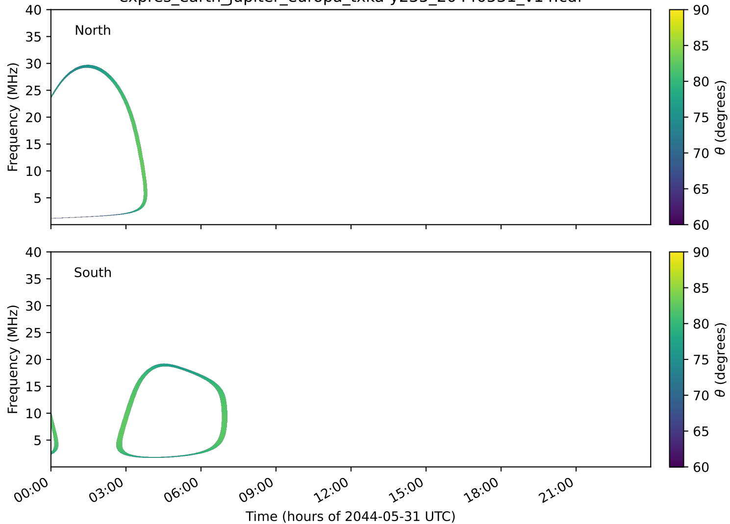
expres_earth_jupiter_europa_txka-y235_20440531_v14.cdf
