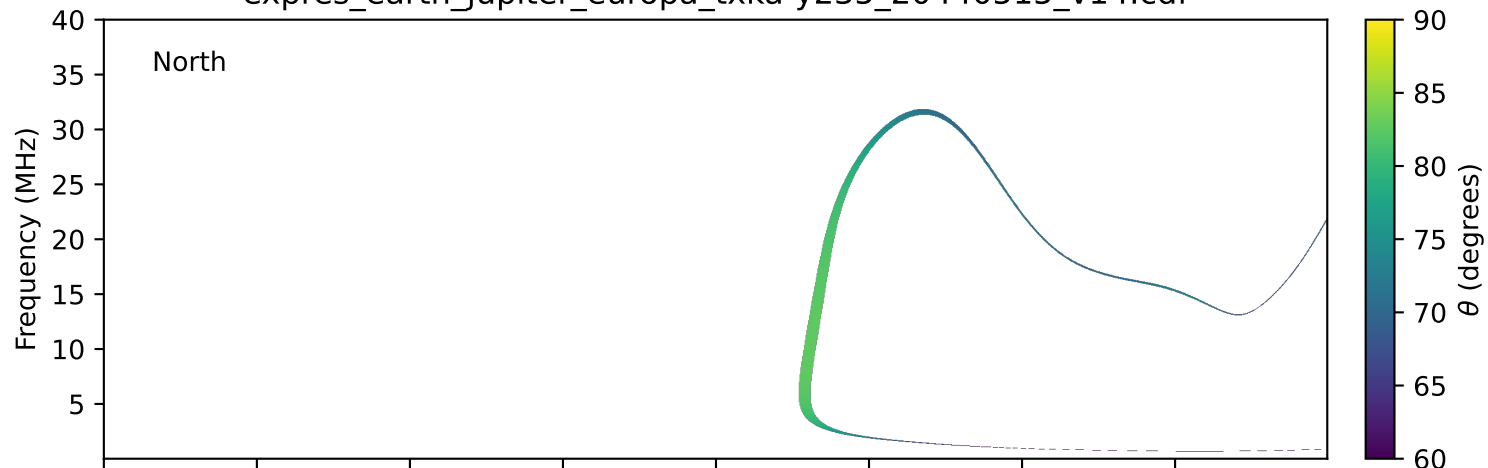
expres_earth_jupiter_europa_txka-y235_20440515_v14.cdf
