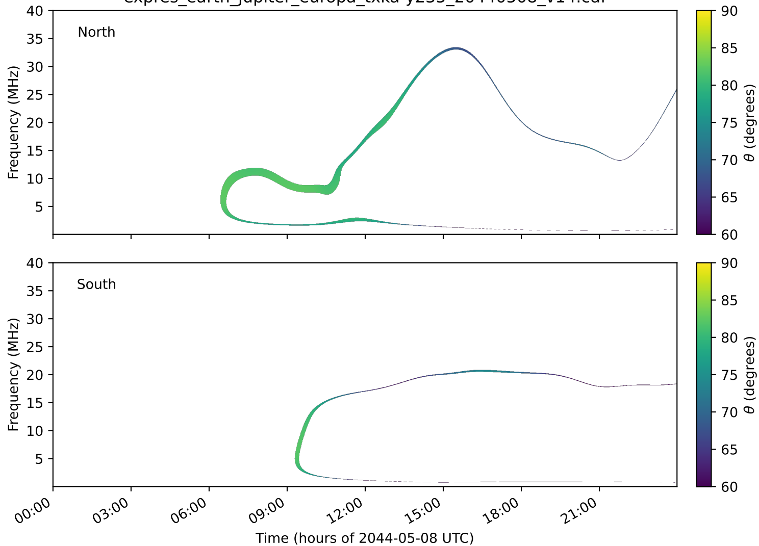
expres_earth_jupiter_europa_txka-y235_20440508_v14.cdf
