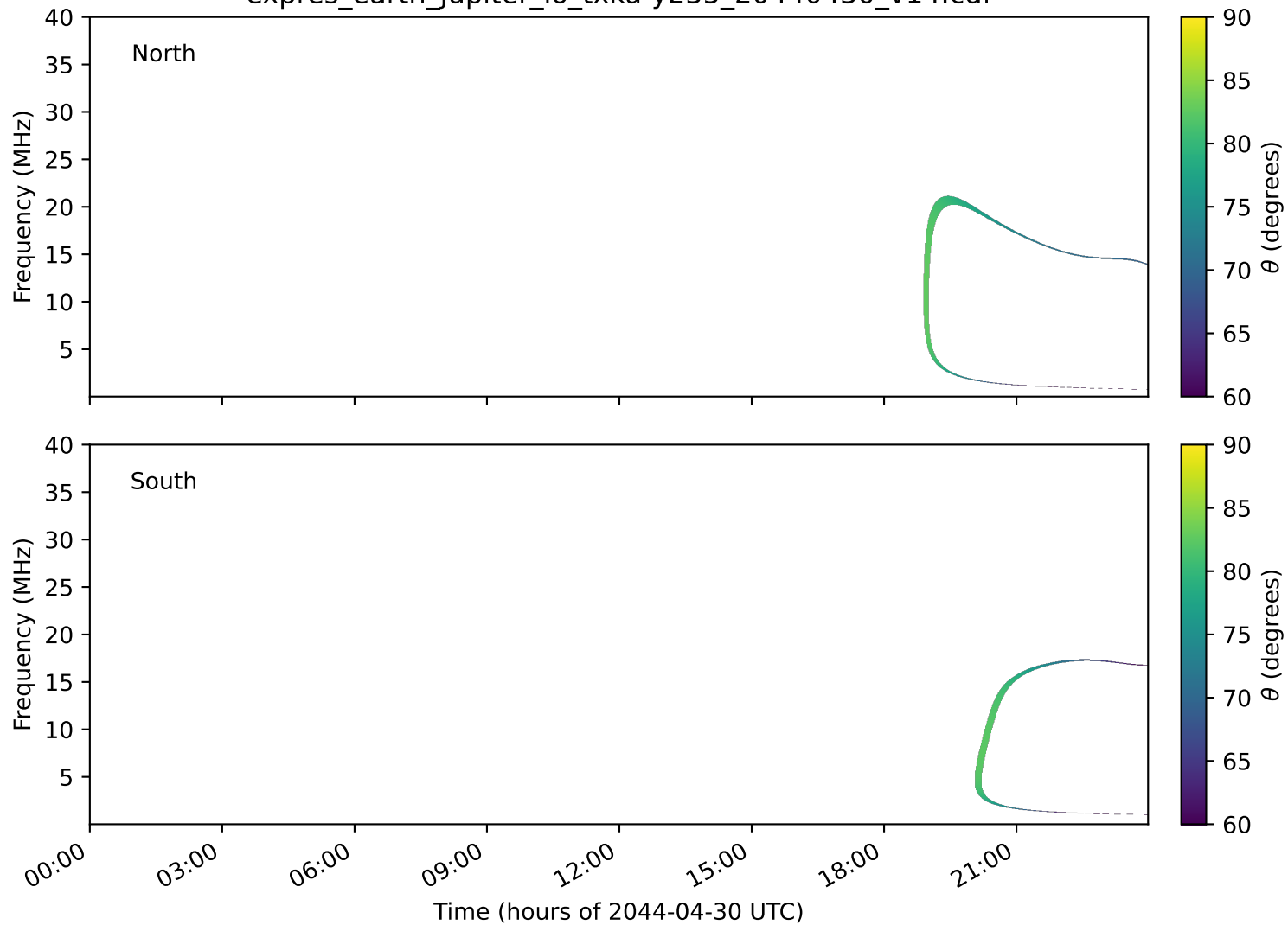
expres_earth_jupiter_io_txka-y235_20440430_v14.cdf
