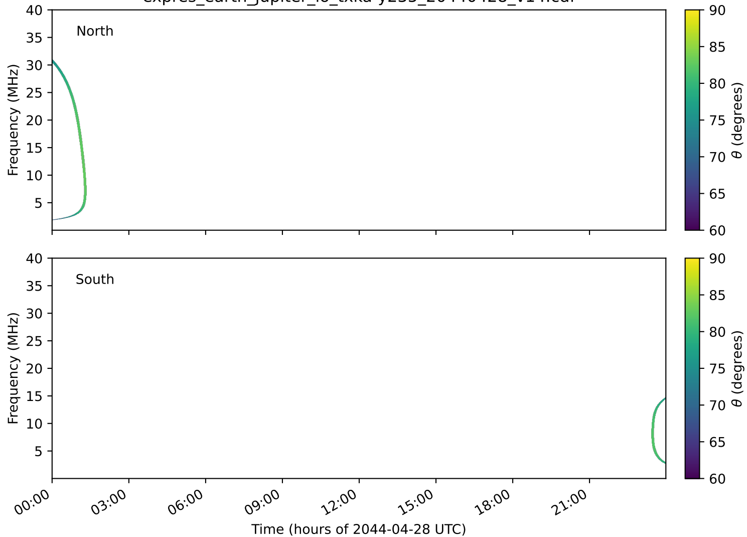
expres_earth_jupiter_io_txka-y235_20440428_v14.cdf
