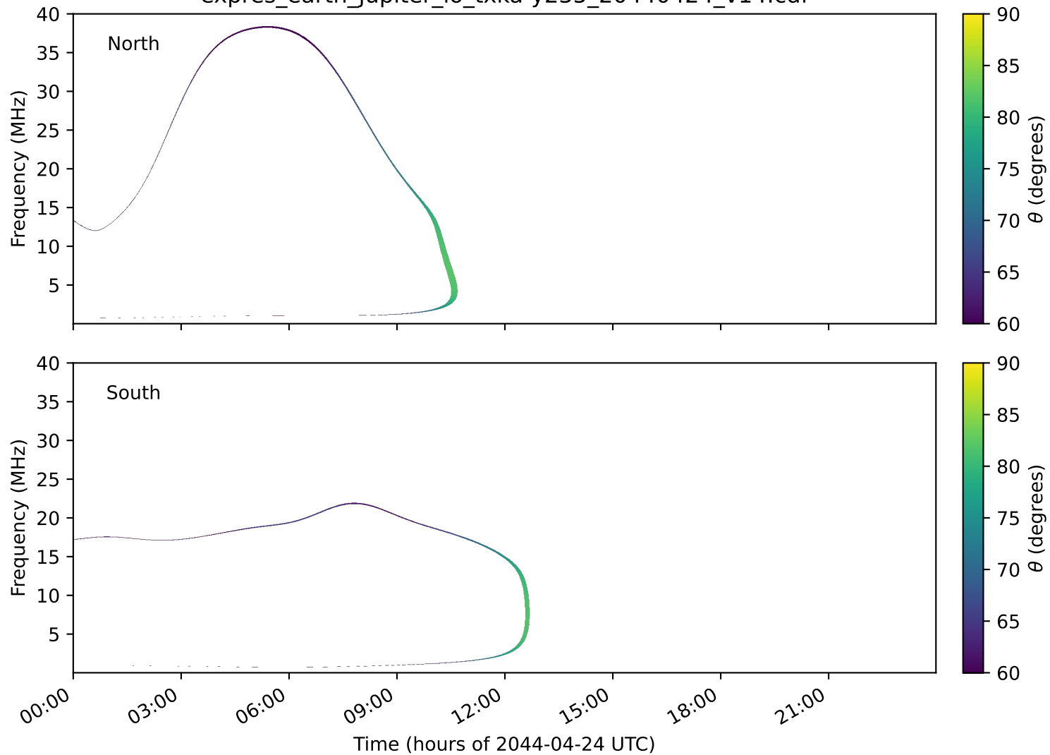
expres_earth_jupiter_io_txka-y235_20440424_v14.cdf
