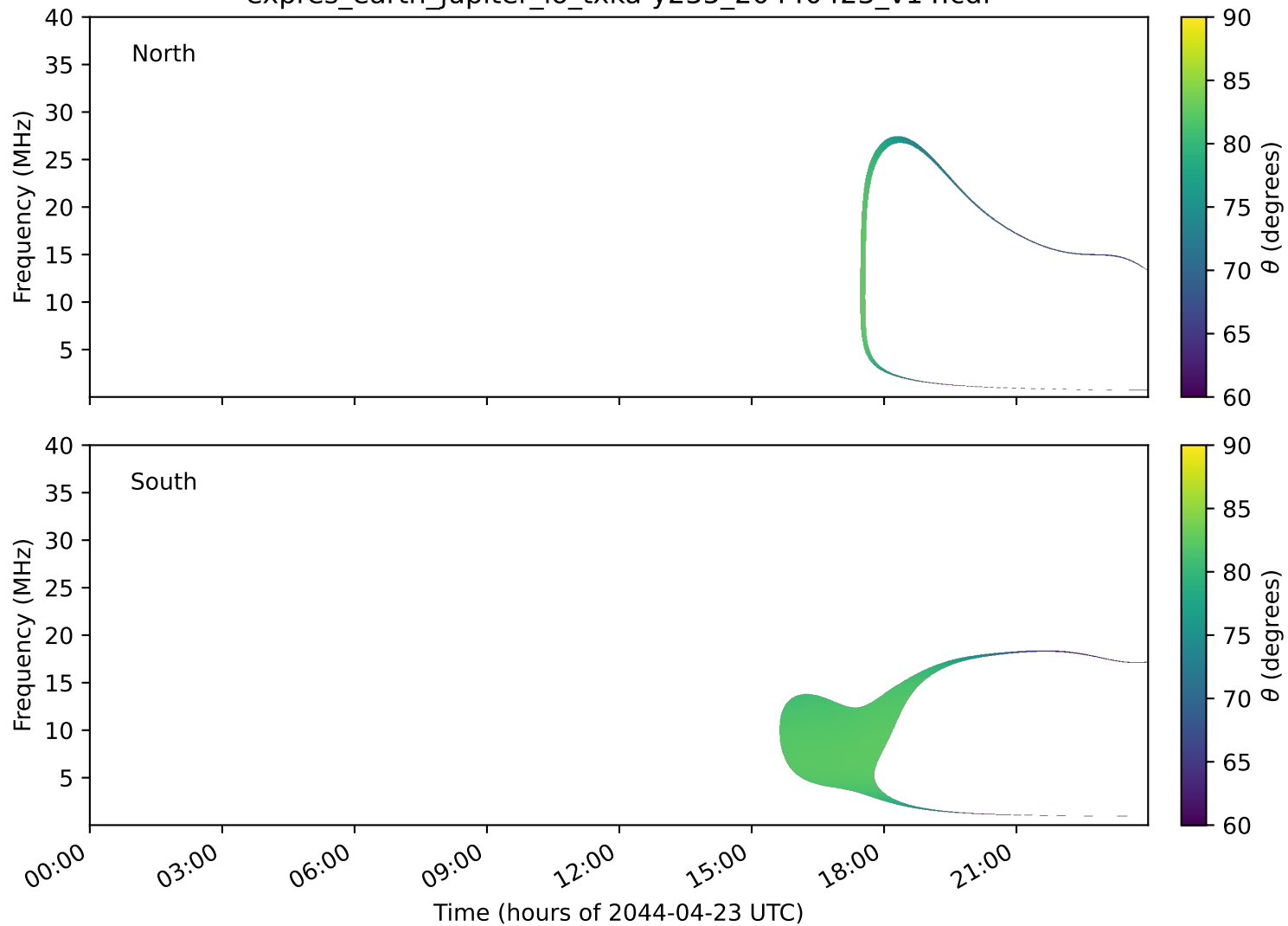
expres_earth_jupiter_io_txka-y235_20440423_v14.cdf
