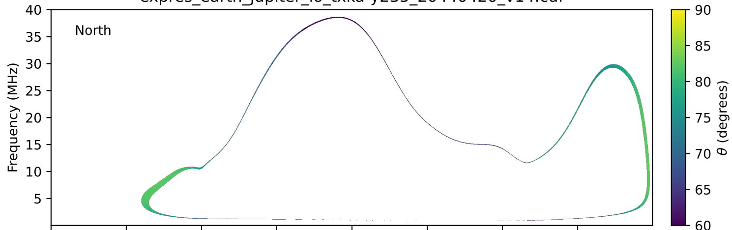
expres_earth_jupiter_io_txka-y235_20440420_v14.cdf
