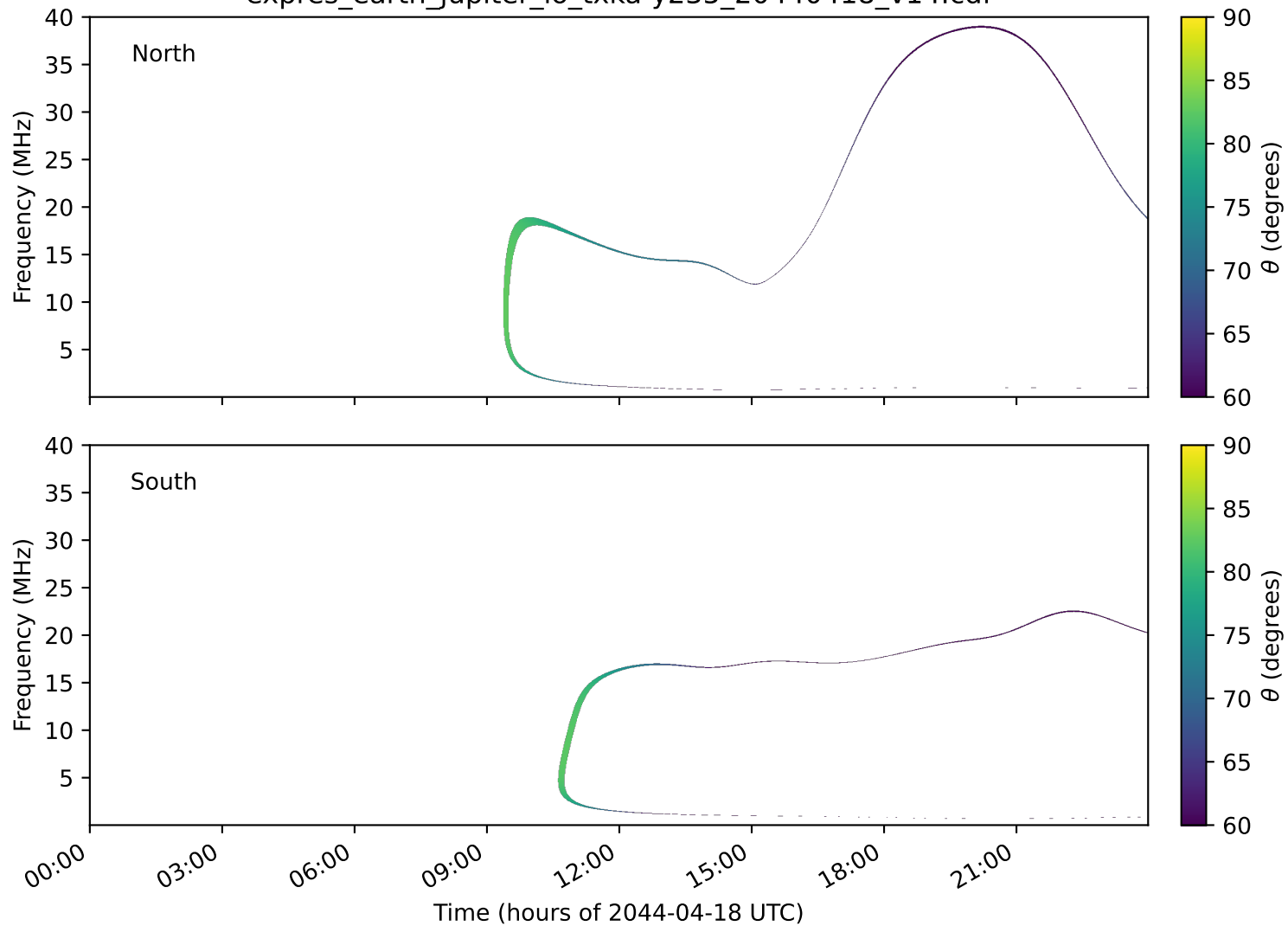
expres_earth_jupiter_io_txka-y235_20440418_v14.cdf
