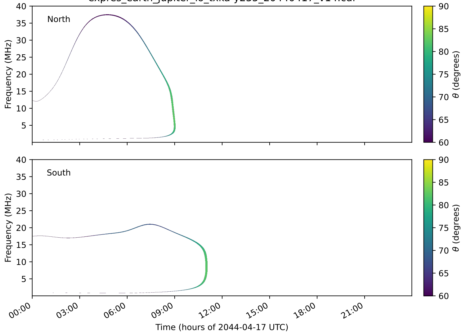
expres_earth_jupiter_io_txka-y235_20440417_v14.cdf
