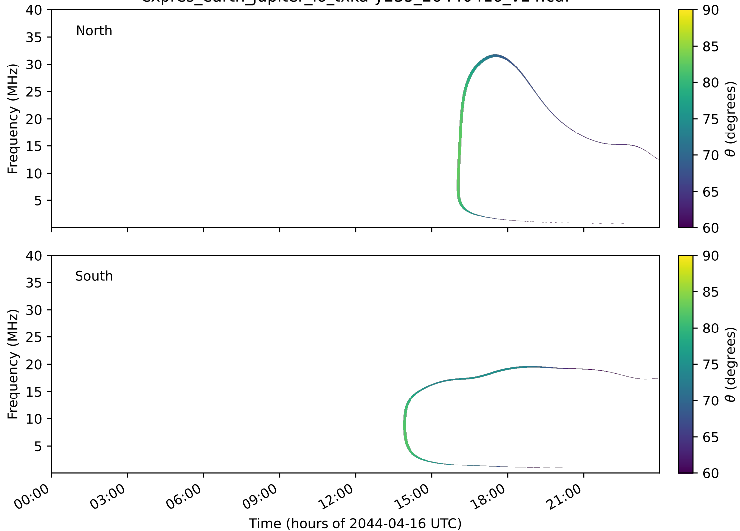
expres_earth_jupiter_io_txka-y235_20440416_v14.cdf
