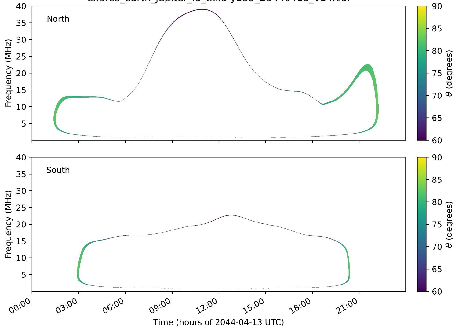
expres_earth_jupiter_io_txka-y235_20440413_v14.cdf
