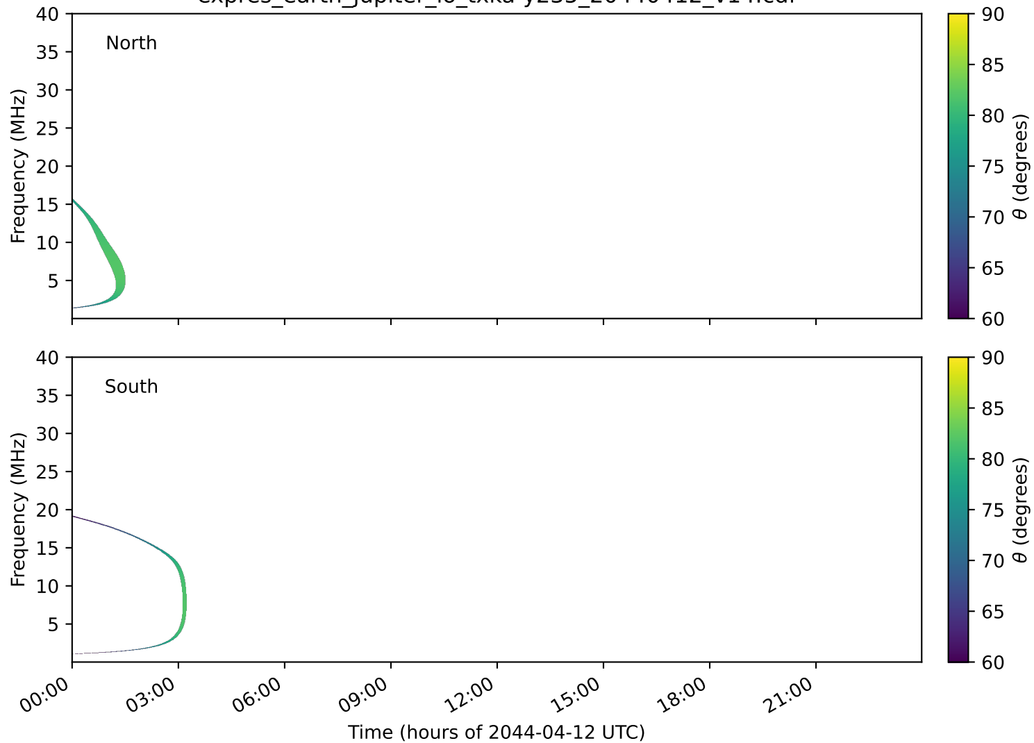
expres_earth_jupiter_io_txka-y235_20440412_v14.cdf
