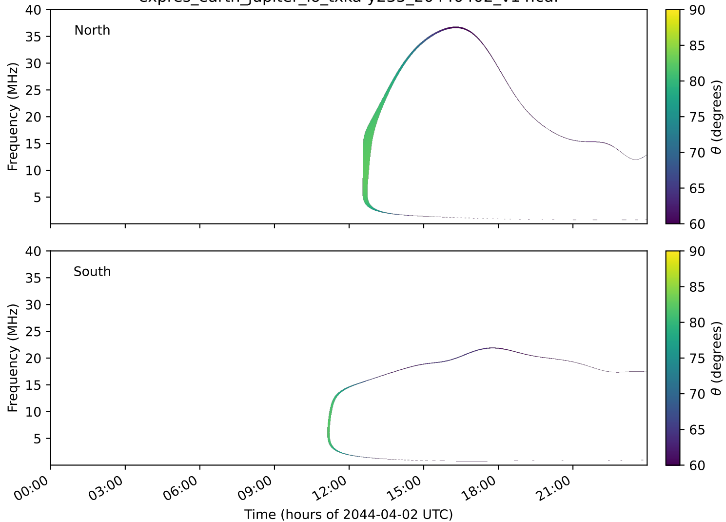
expres_earth_jupiter_io_txka-y235_20440402_v14.cdf
