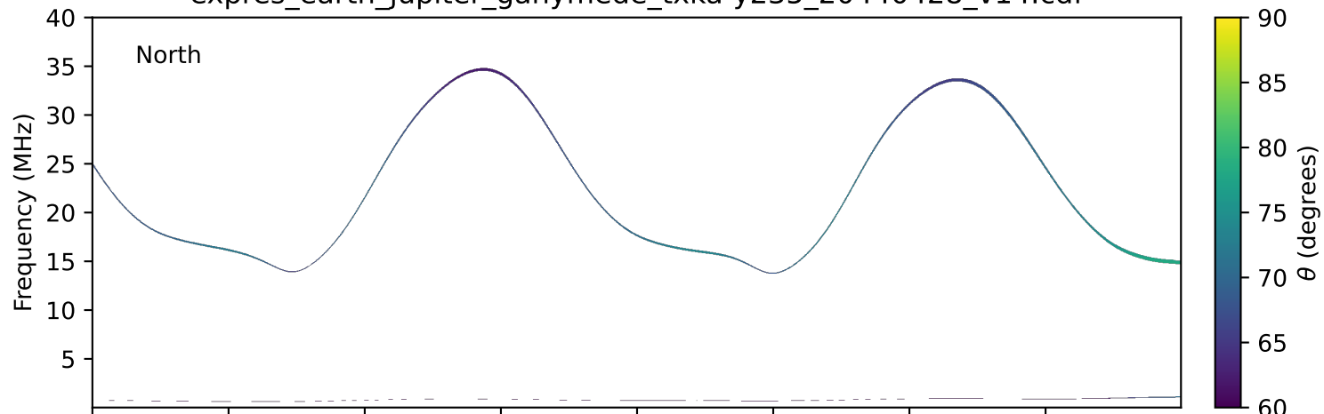
expres_earth_jupiter_ganymede_txka-y235_20440428_v14.cdf
