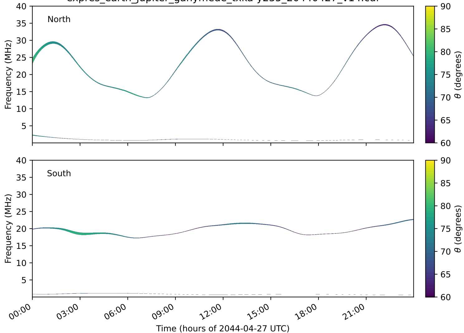
expres_earth_jupiter_ganymede_txka-y235_20440427_v14.cdf
