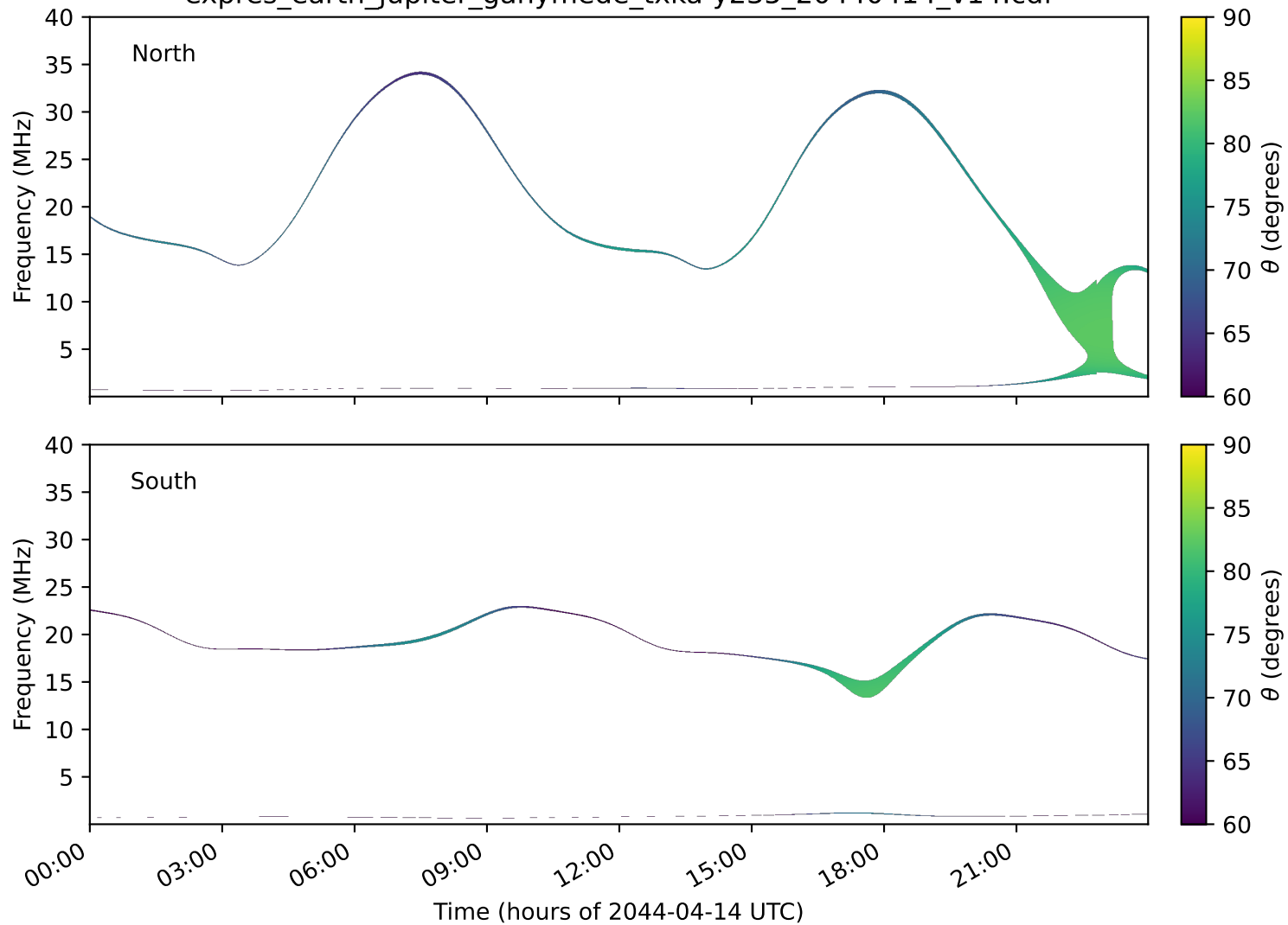
expres_earth_jupiter_ganymede_txka-y235_20440414_v14.cdf
