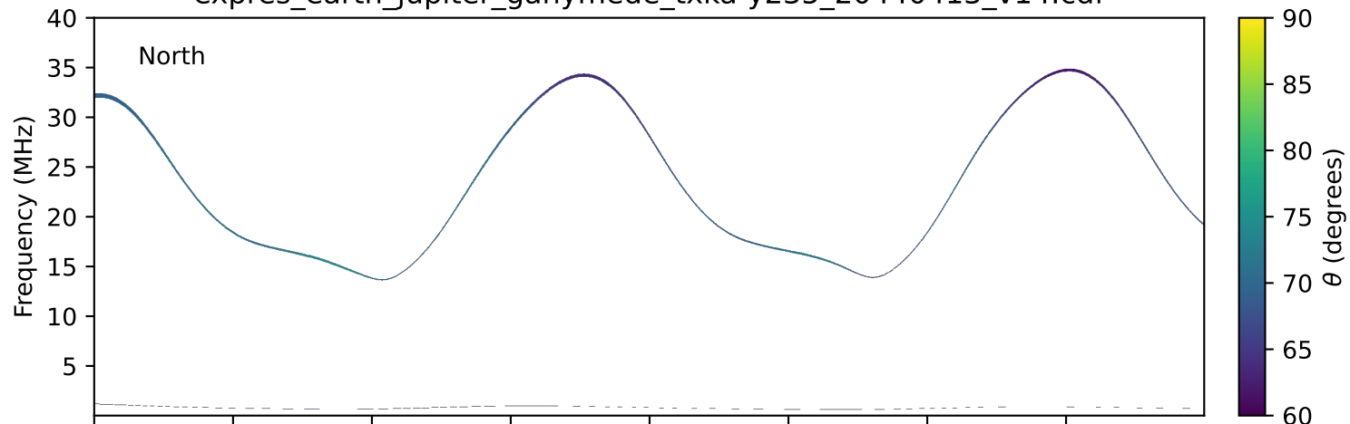
expres_earth_jupiter_ganymede_txka-y235_20440413_v14.cdf
