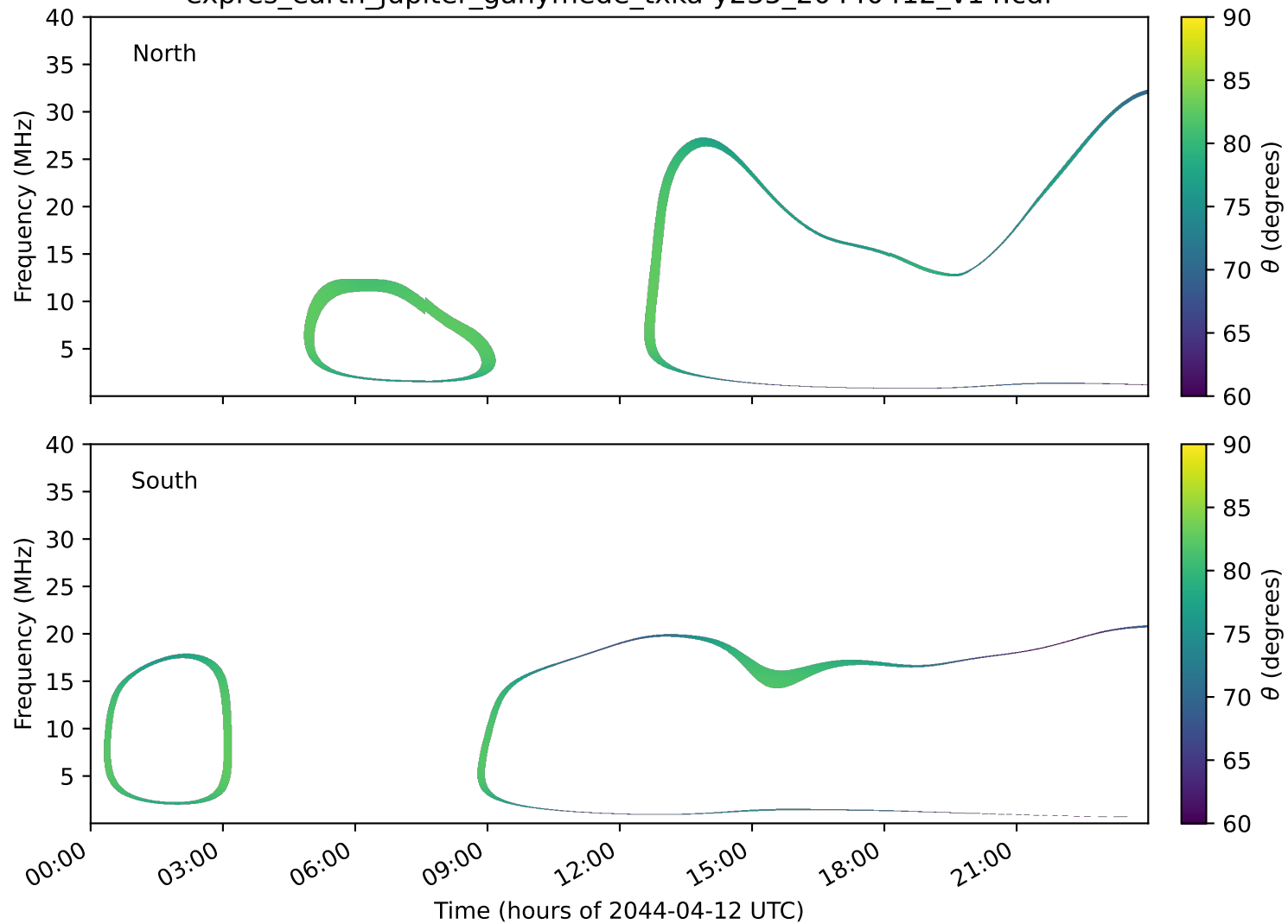
expres_earth_jupiter_ganymede_txka-y235_20440412_v14.cdf
