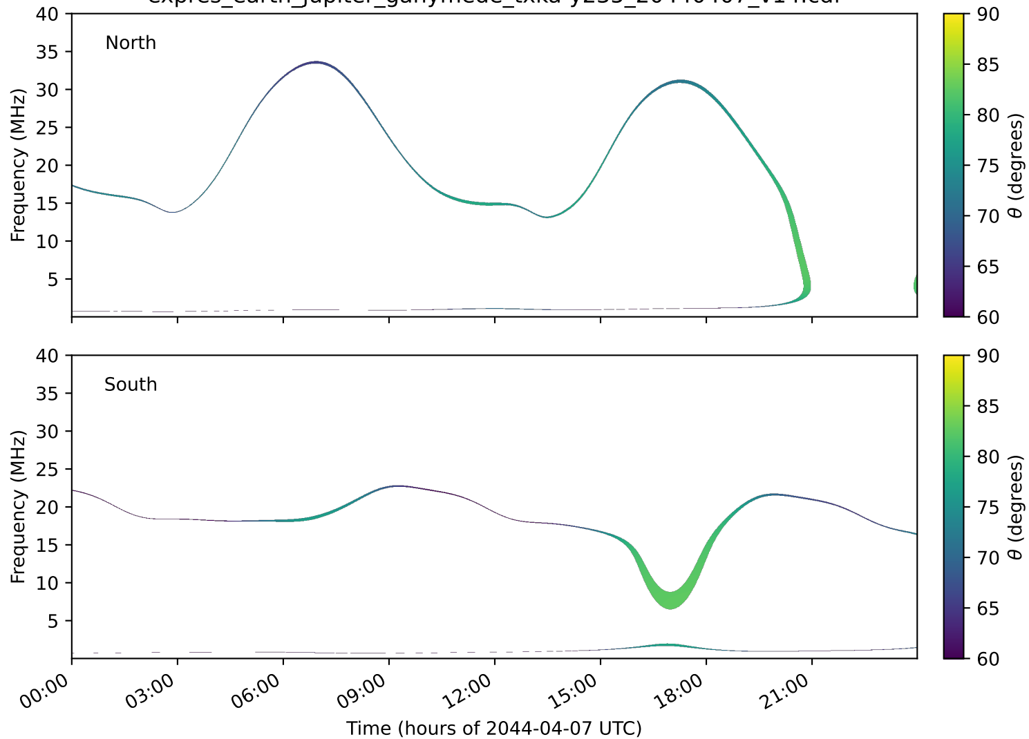
expres_earth_jupiter_ganymede_txka-y235_20440407_v14.cdf
