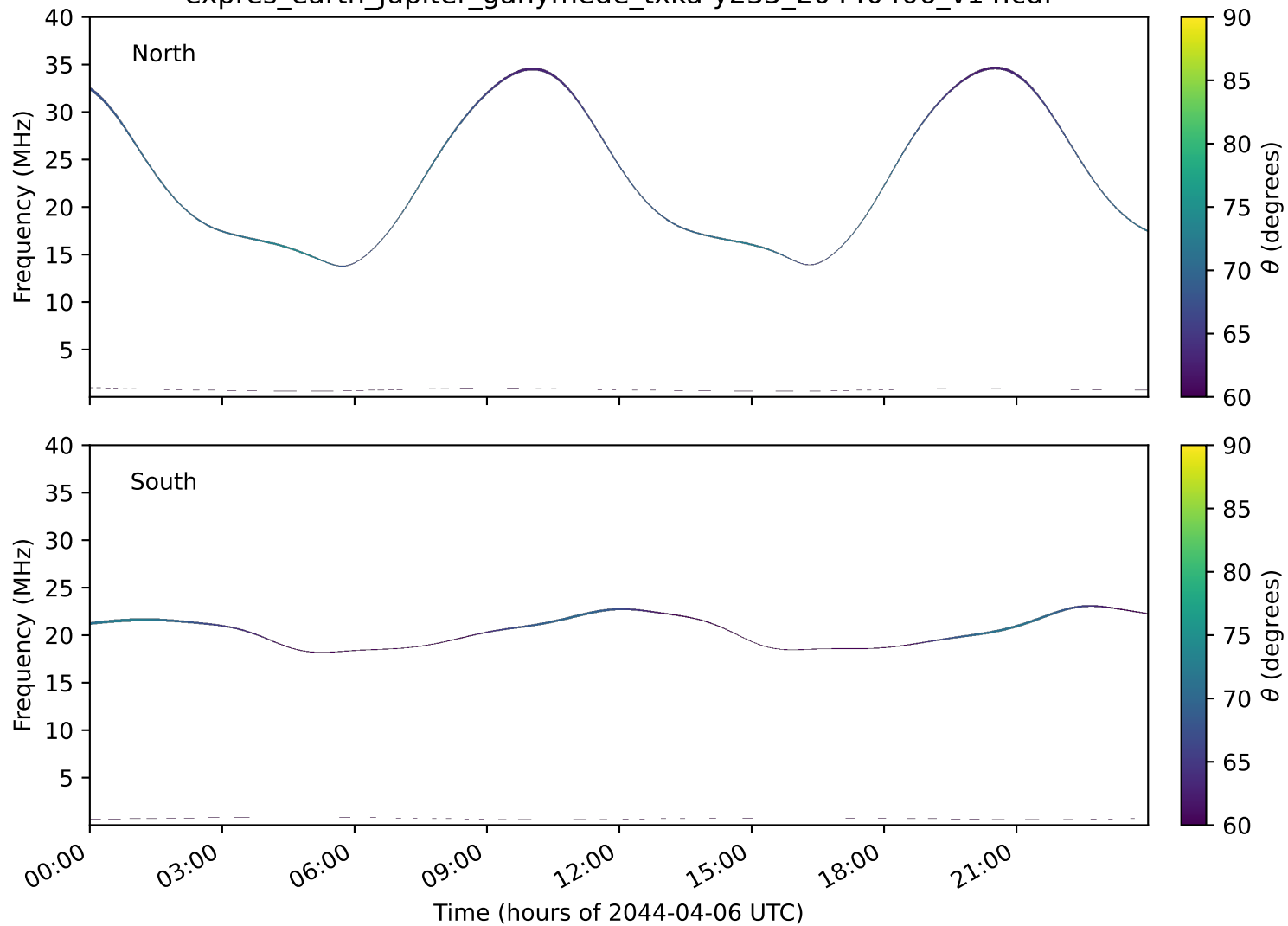
expres_earth_jupiter_ganymede_txka-y235_20440406_v14.cdf
