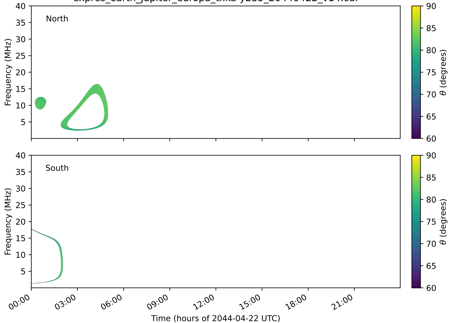
expres_earth_jupiter_europa_txka-y235_20440422_v14.cdf
