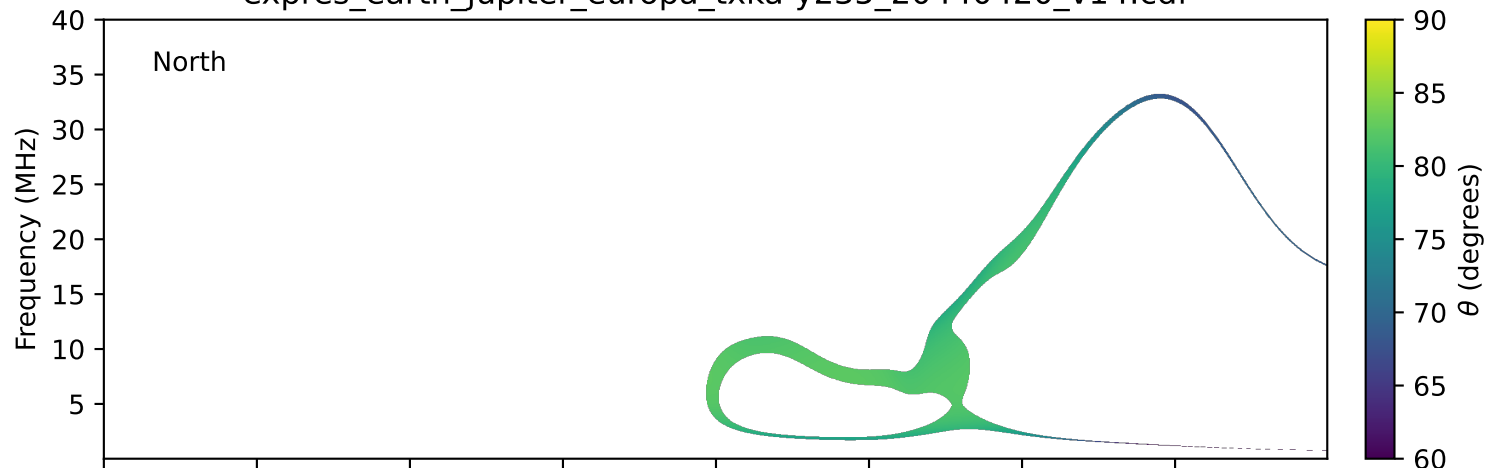
expres_earth_jupiter_europa_txka-y235_20440420_v14.cdf
