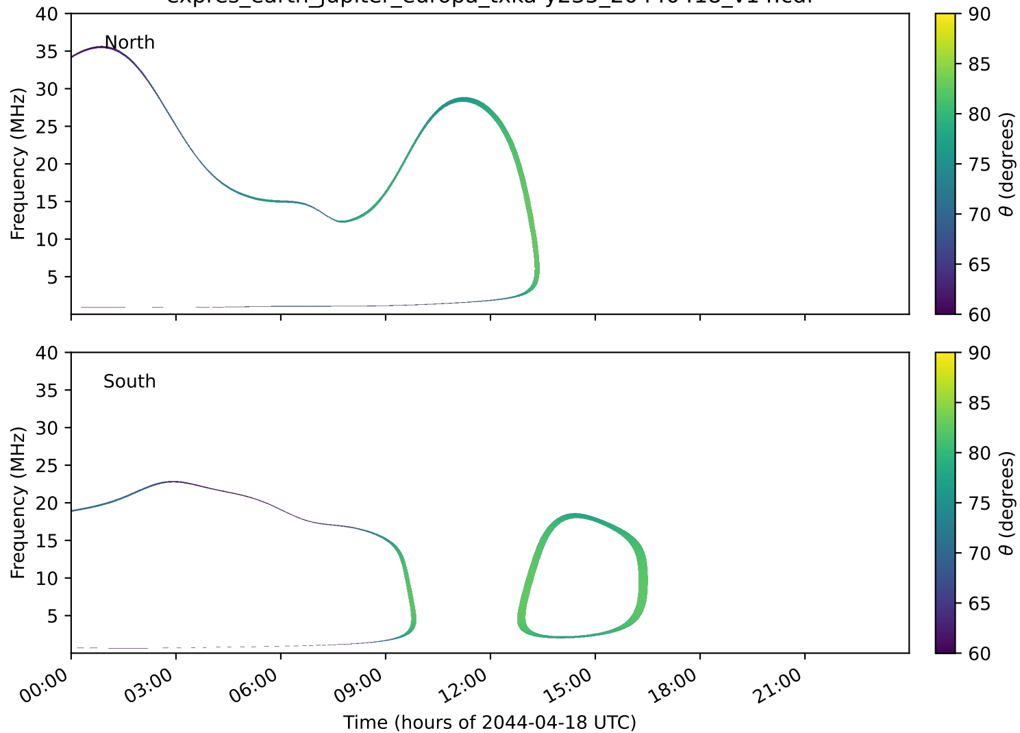
expres_earth_jupiter_europa_txka-y235_20440418_v14.cdf
