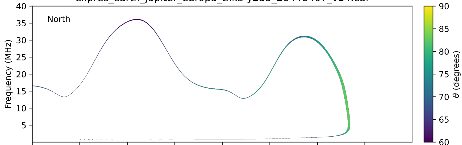
expres_earth_jupiter_europa_txka-y235_20440407_v14.cdf
