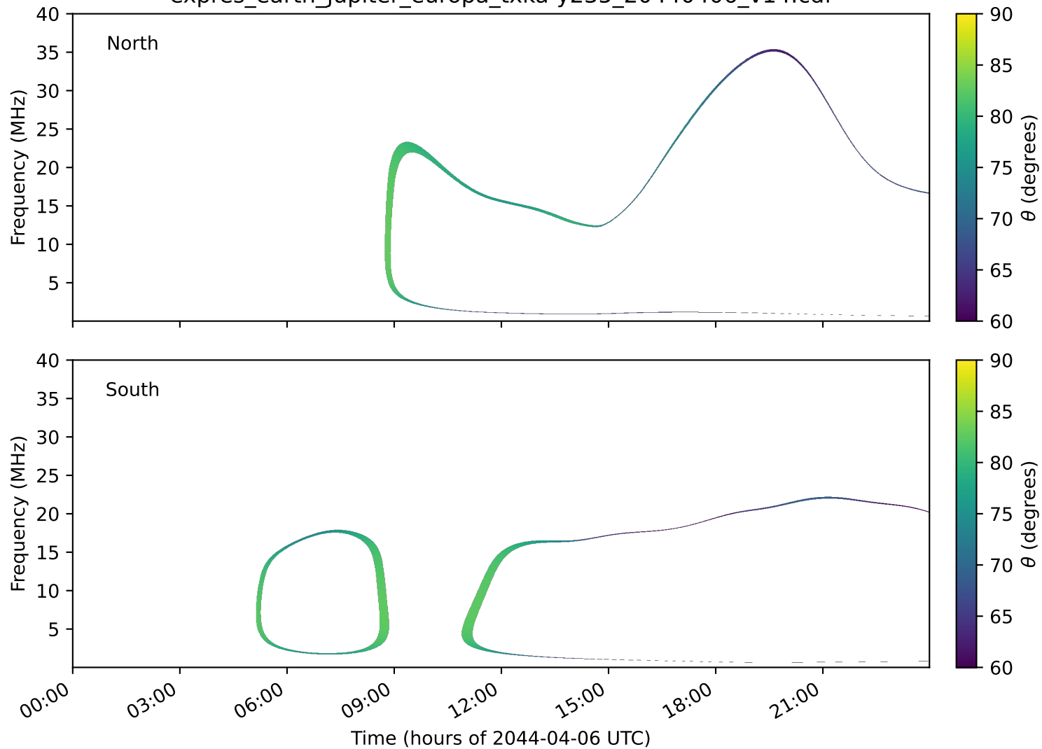
expres_earth_jupiter_europa_txka-y235_20440406_v14.cdf
