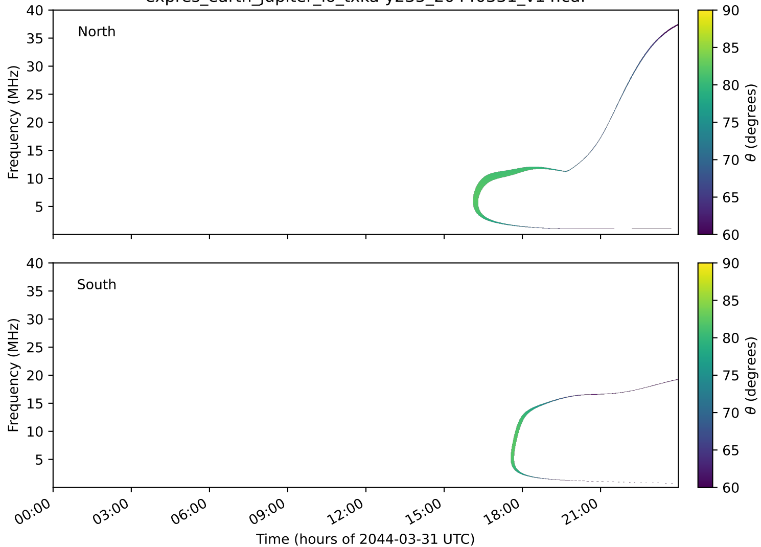
expres_earth_jupiter_io_txka-y235_20440331_v14.cdf
