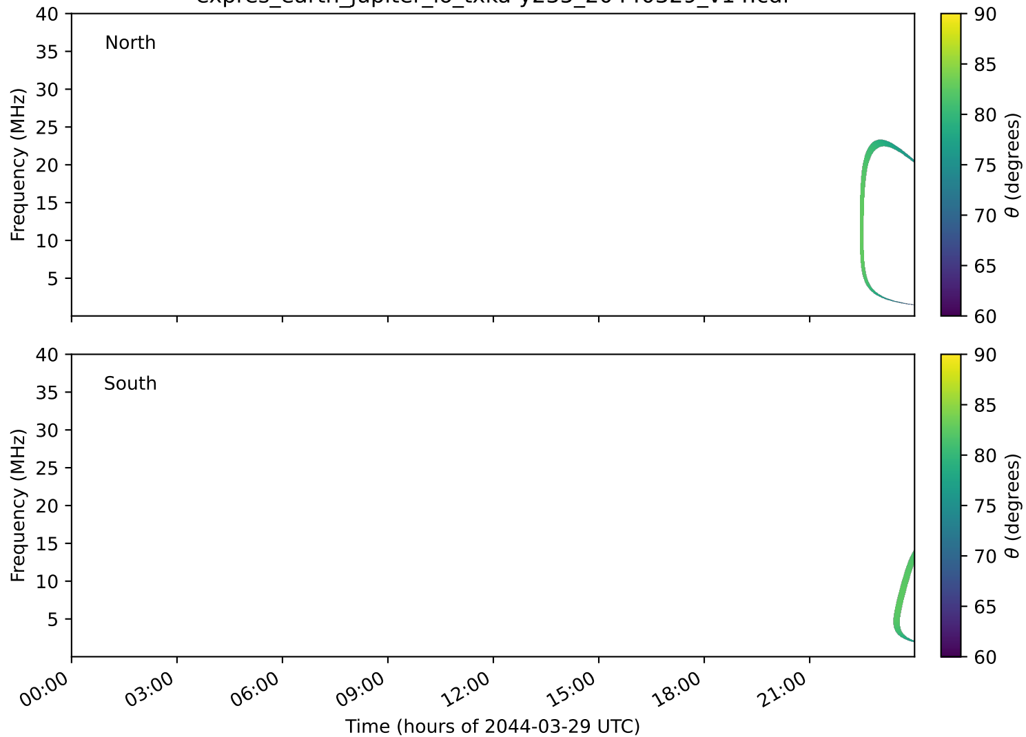
expres_earth_jupiter_io_txka-y235_20440329_v14.cdf
