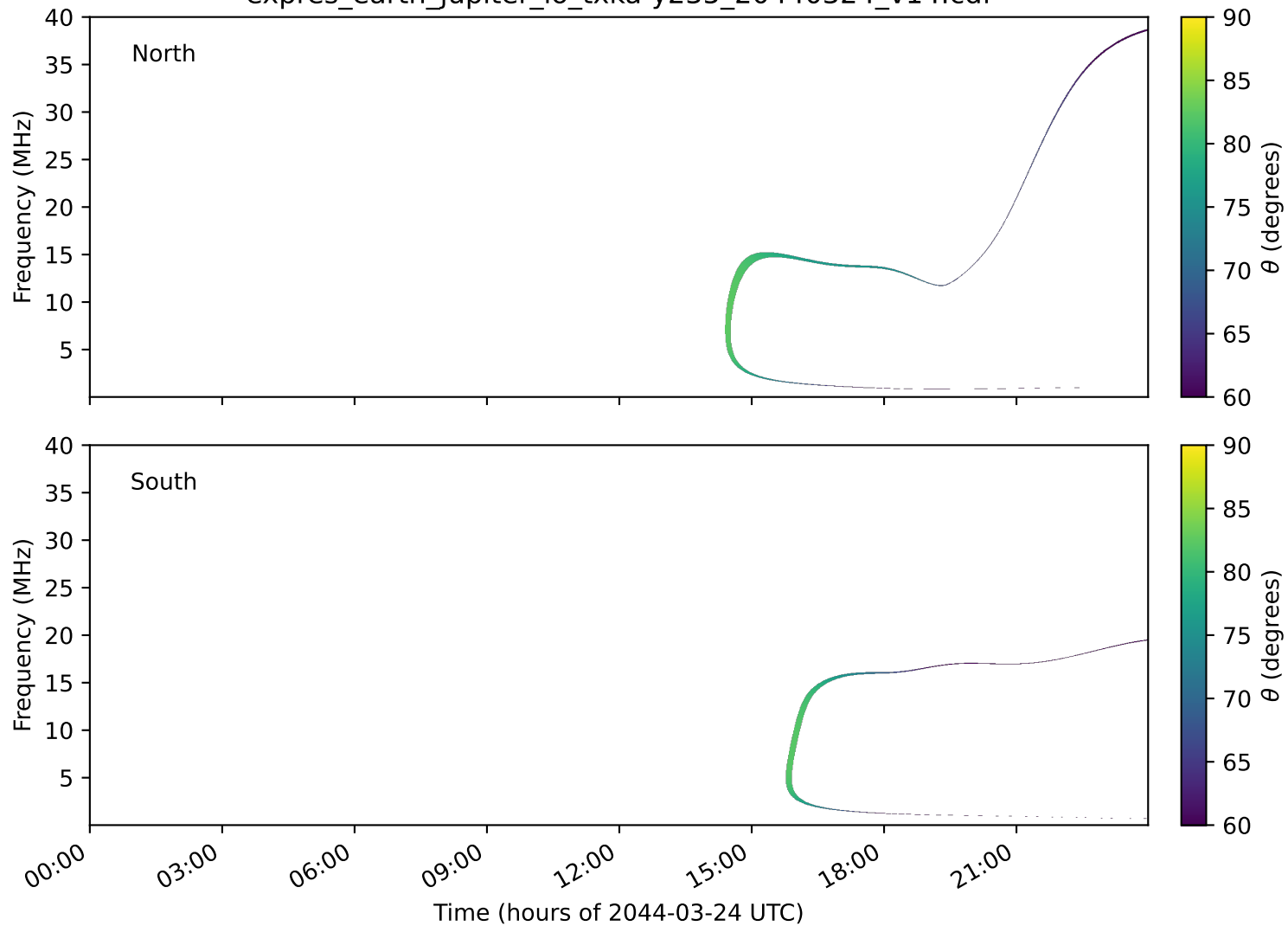
expres_earth_jupiter_io_txka-y235_20440324_v14.cdf
