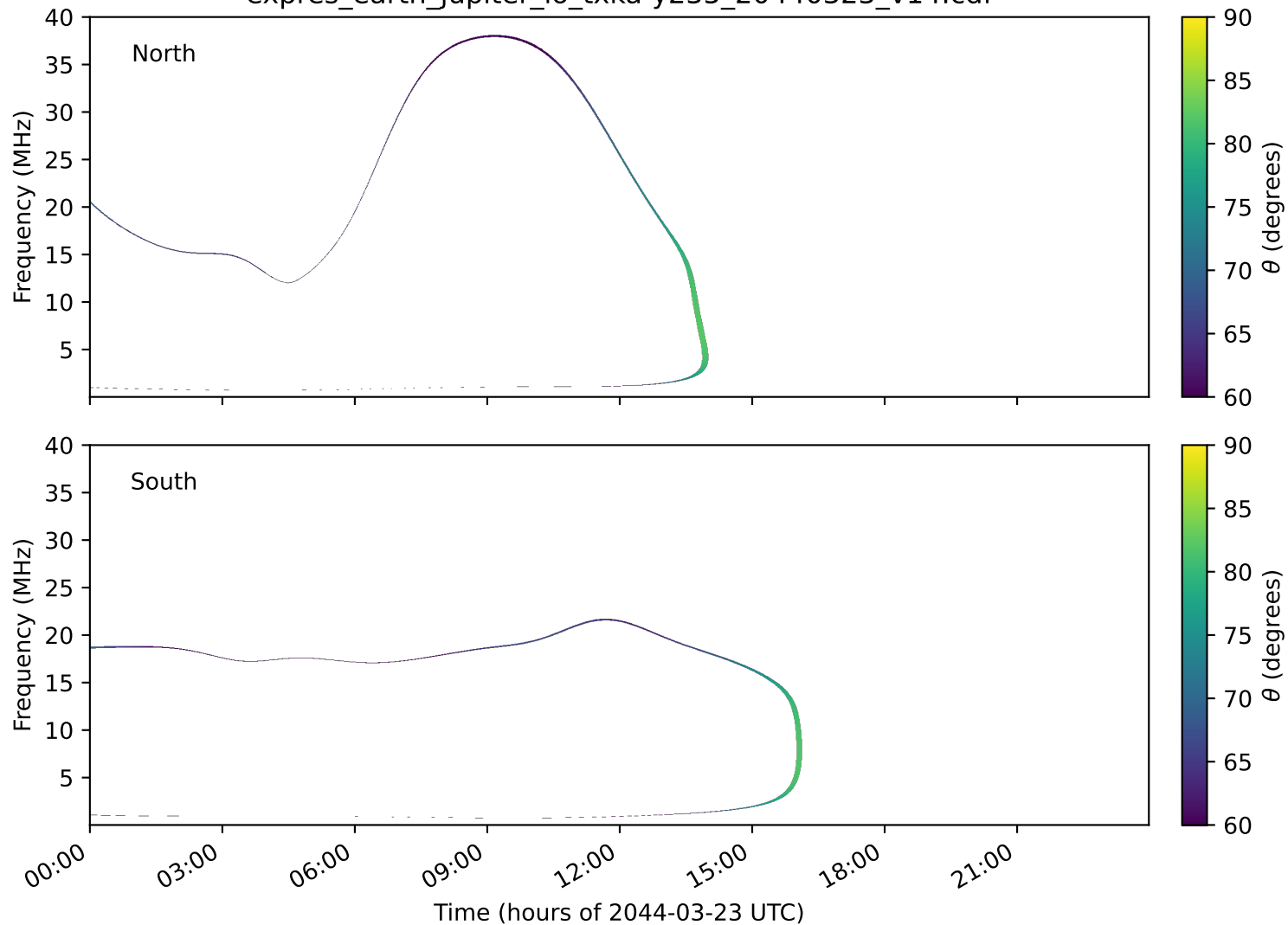
expres_earth_jupiter_io_txka-y235_20440323_v14.cdf
