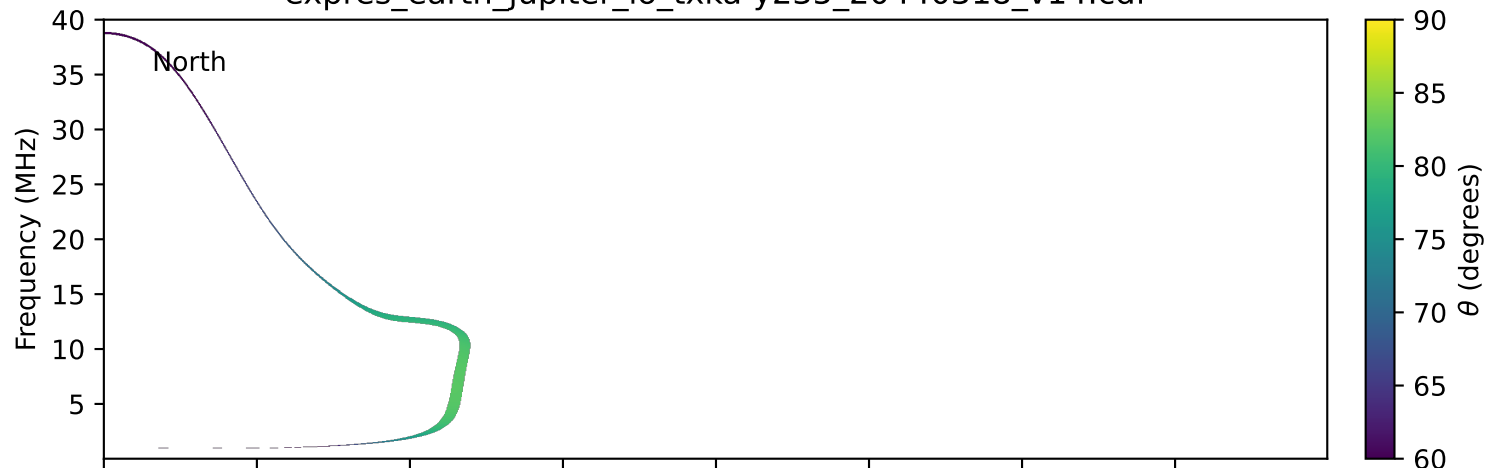
expres_earth_jupiter_io_txka-y235_20440318_v14.cdf
