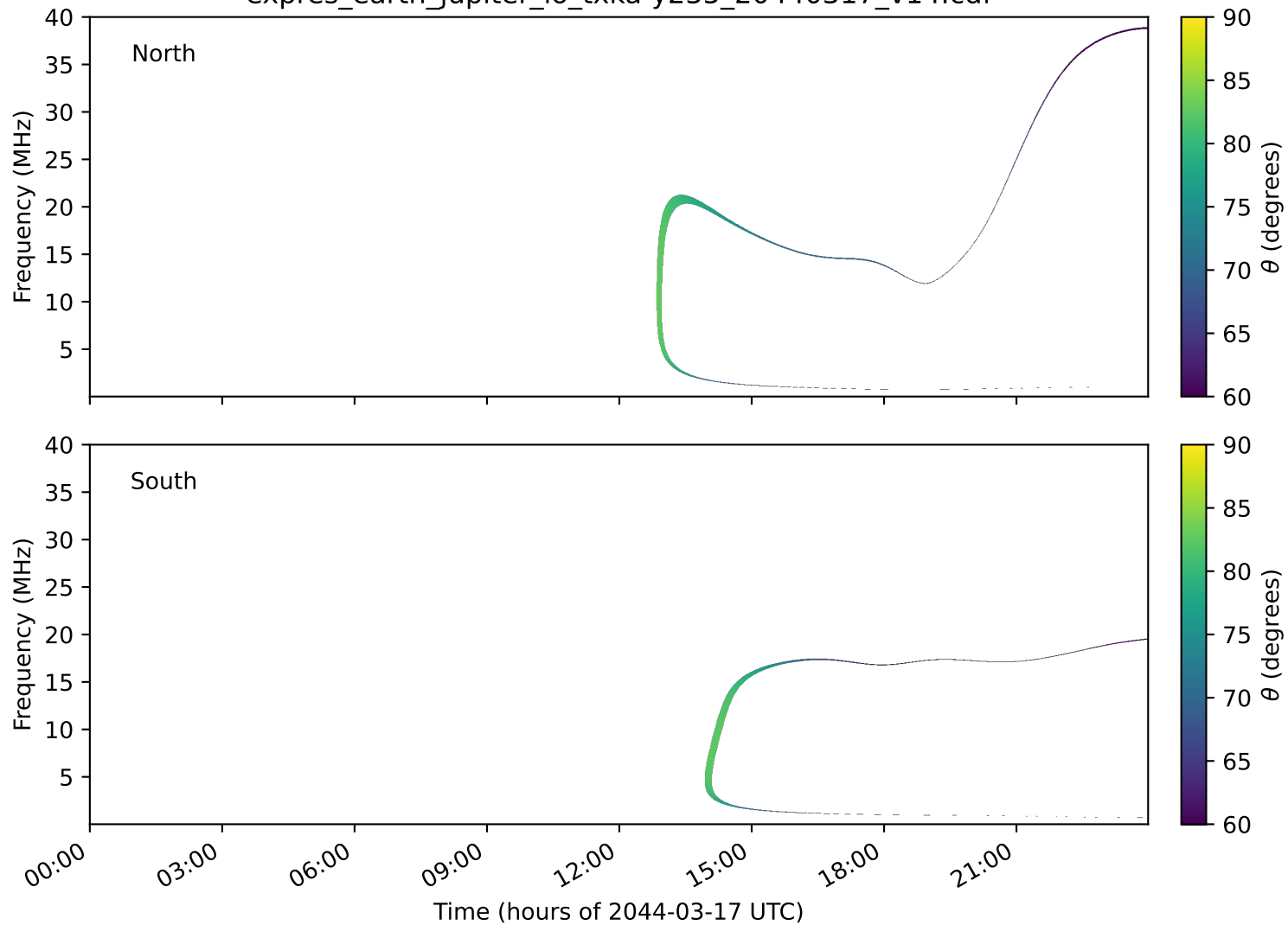
expres_earth_jupiter_io_txka-y235_20440317_v14.cdf
