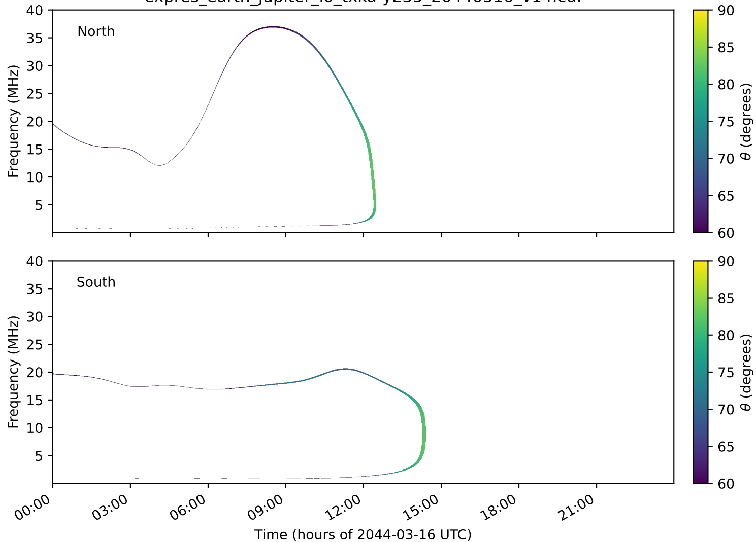
expres_earth_jupiter_io_txka-y235_20440316_v14.cdf
