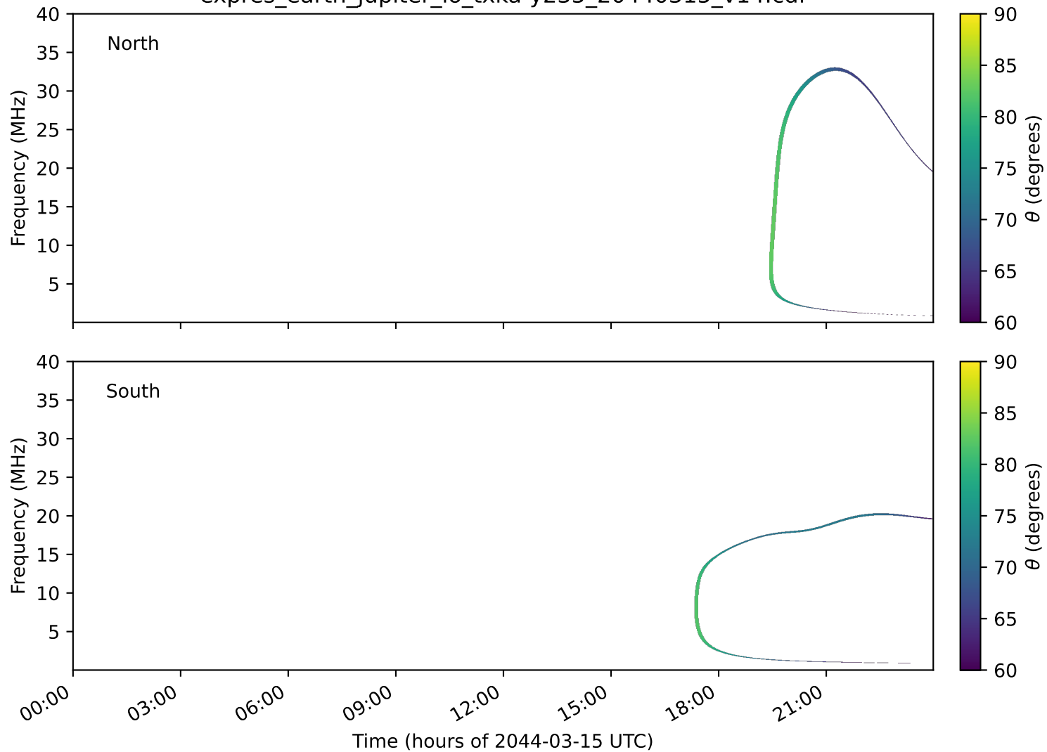
expres_earth_jupiter_io_txka-y235_20440315_v14.cdf
