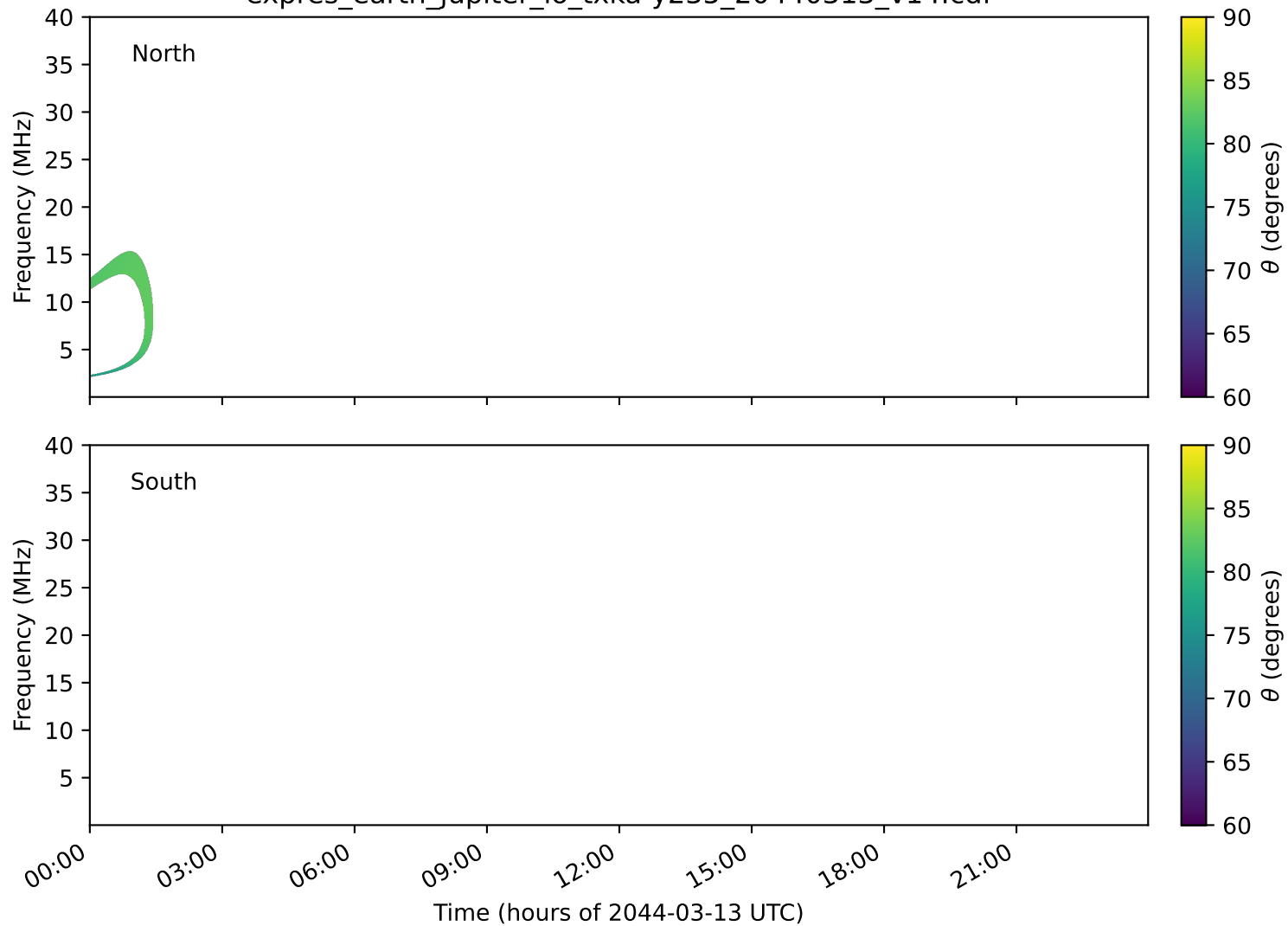
expres_earth_jupiter_io_txka-y235_20440313_v14.cdf
