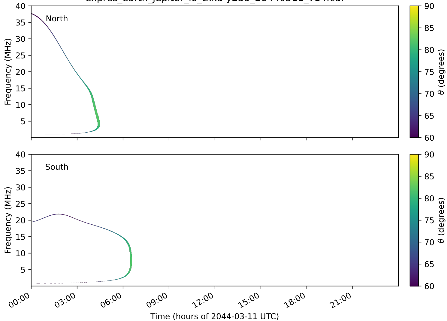
expres_earth_jupiter_io_txka-y235_20440311_v14.cdf
