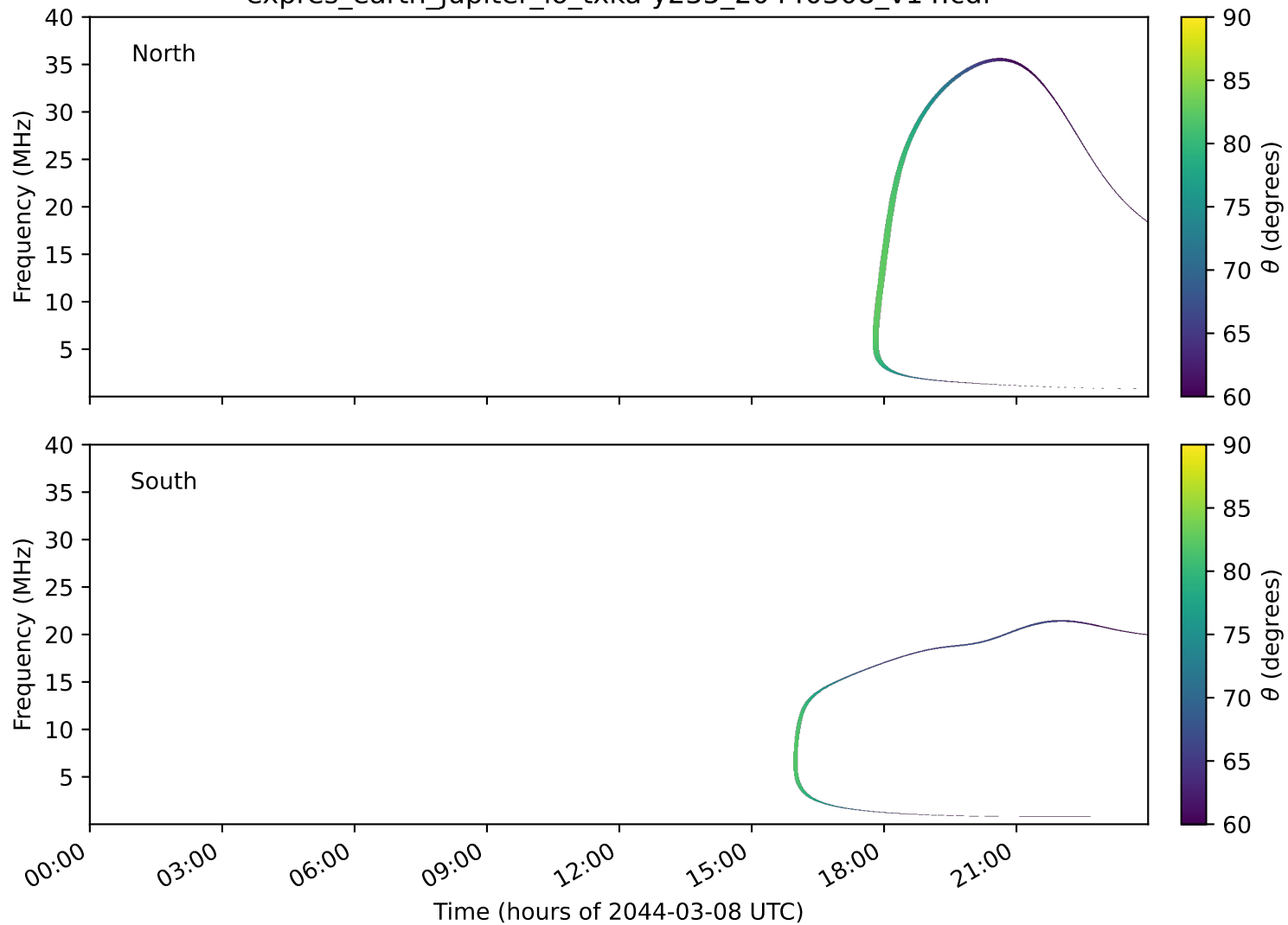
expres_earth_jupiter_io_txka-y235_20440308_v14.cdf
