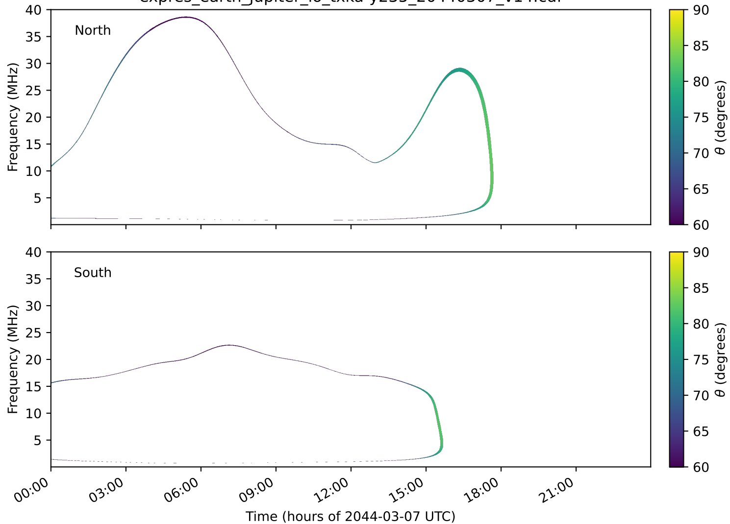
expres_earth_jupiter_io_txka-y235_20440307_v14.cdf
