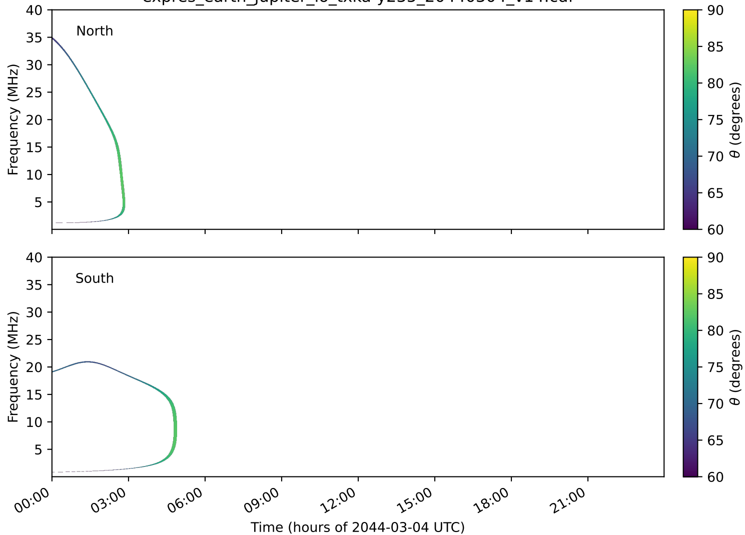
expres_earth_jupiter_io_txka-y235_20440304_v14.cdf
