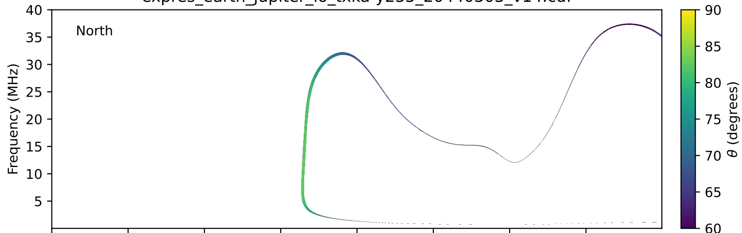
expres_earth_jupiter_io_txka-y235_20440303_v14.cdf
