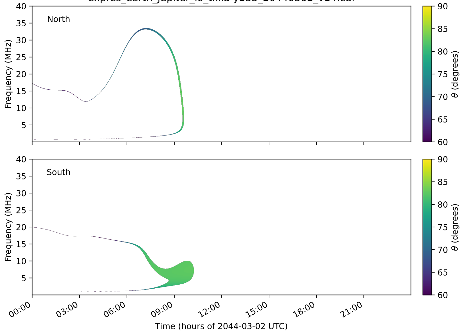
expres_earth_jupiter_io_txka-y235_20440302_v14.cdf
