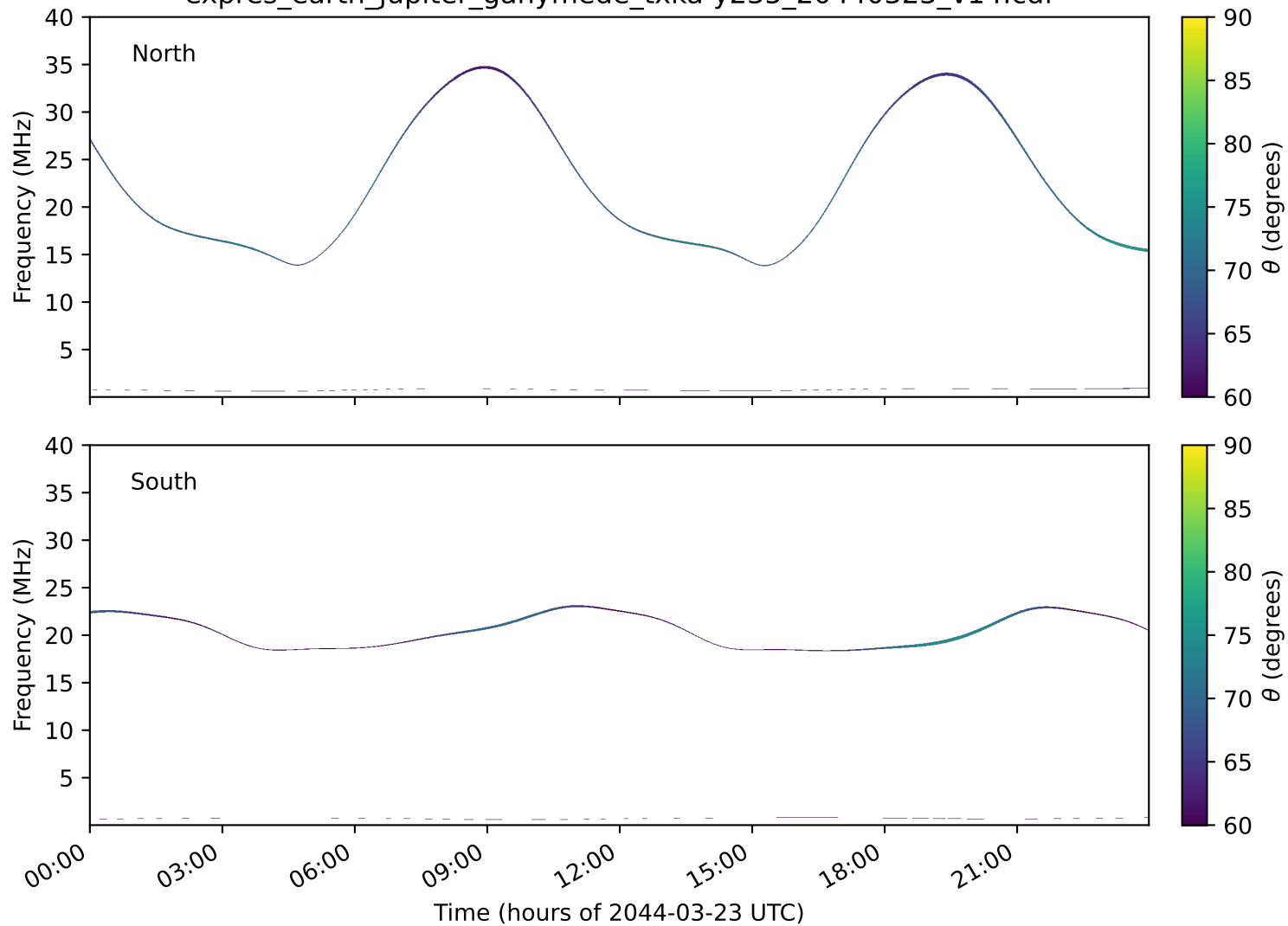
expres_earth_jupiter_ganymede_txka-y235_20440323_v14.cdf
