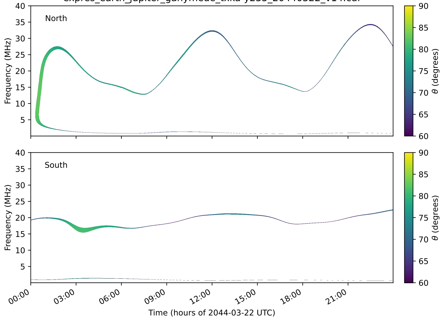
expres_earth_jupiter_ganymede_txka-y235_20440322_v14.cdf
