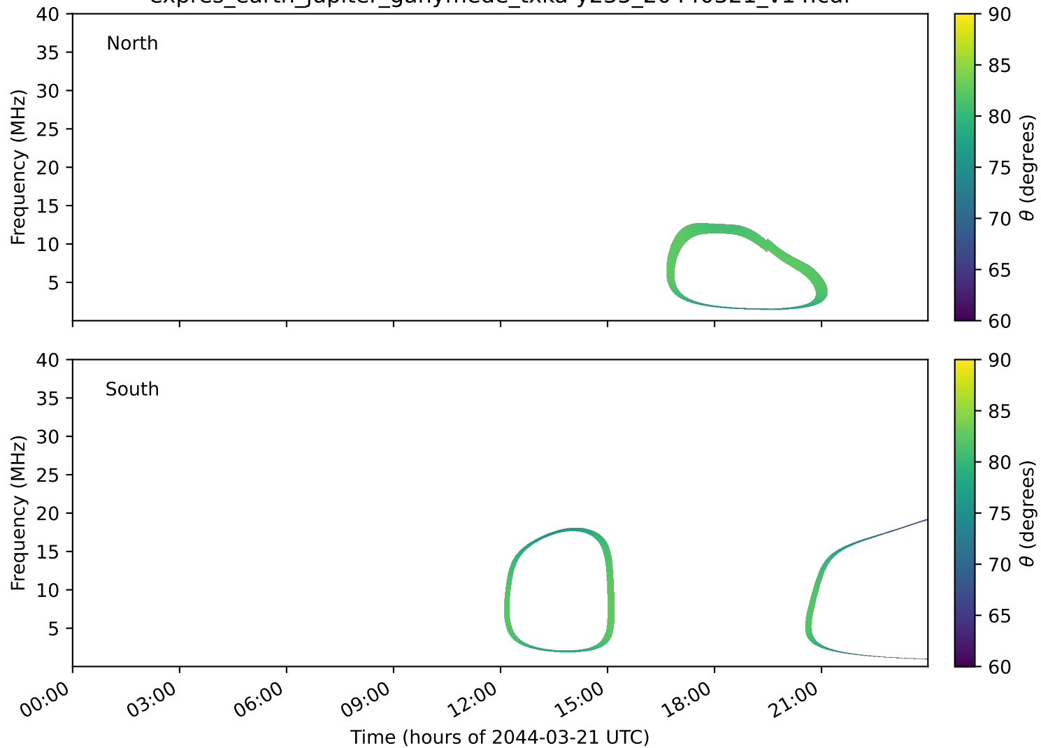
expres_earth_jupiter_ganymede_txka-y235_20440321_v14.cdf
