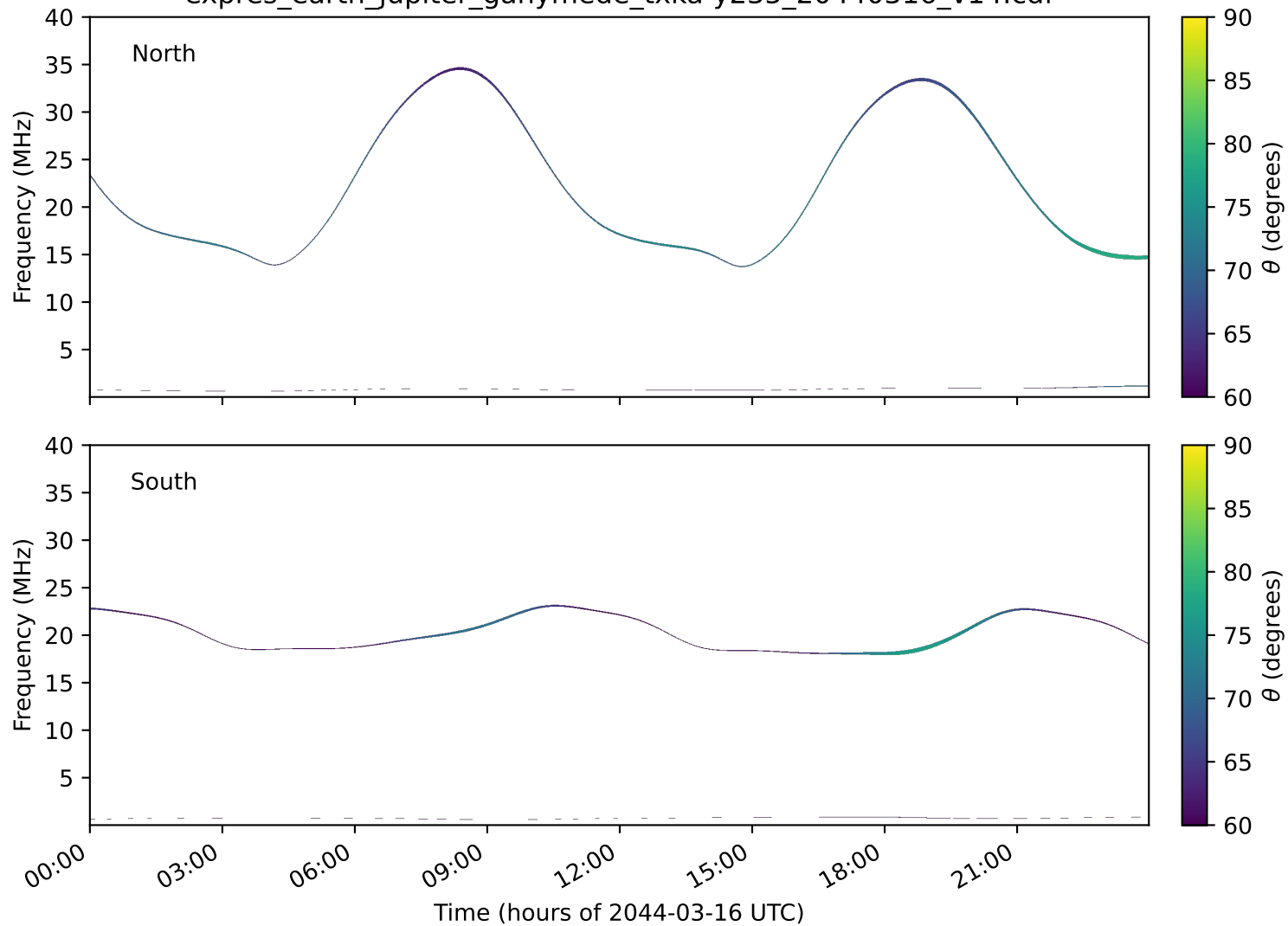
expres_earth_jupiter_ganymede_txka-y235_20440316_v14.cdf
