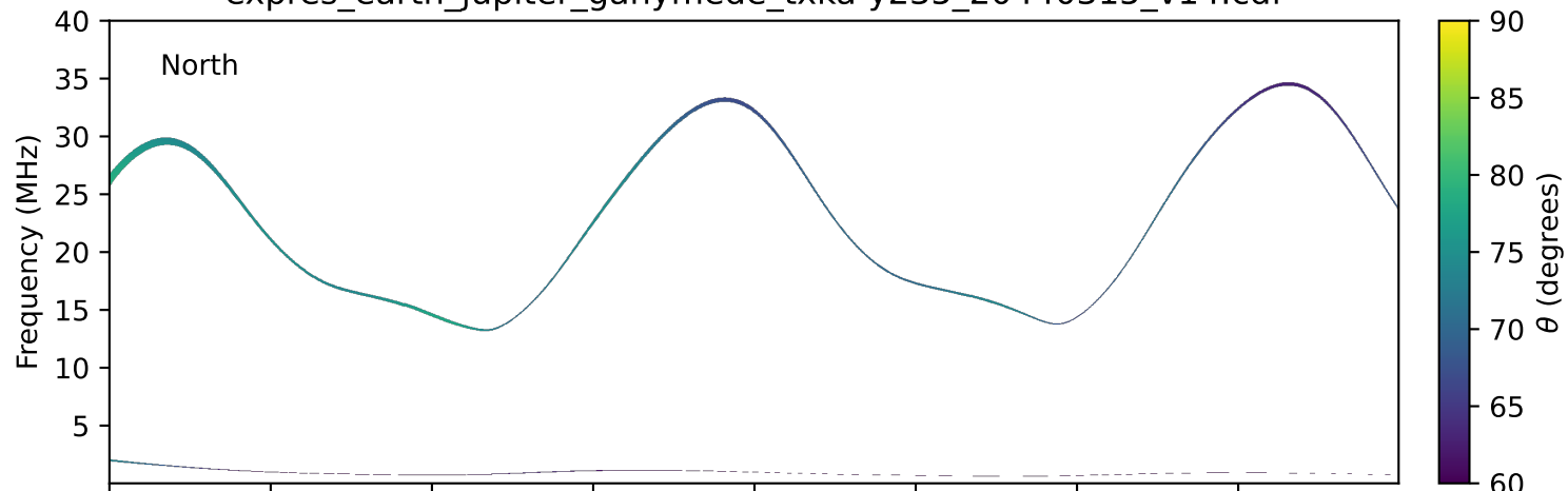
expres_earth_jupiter_ganymede_txka-y235_20440315_v14.cdf
