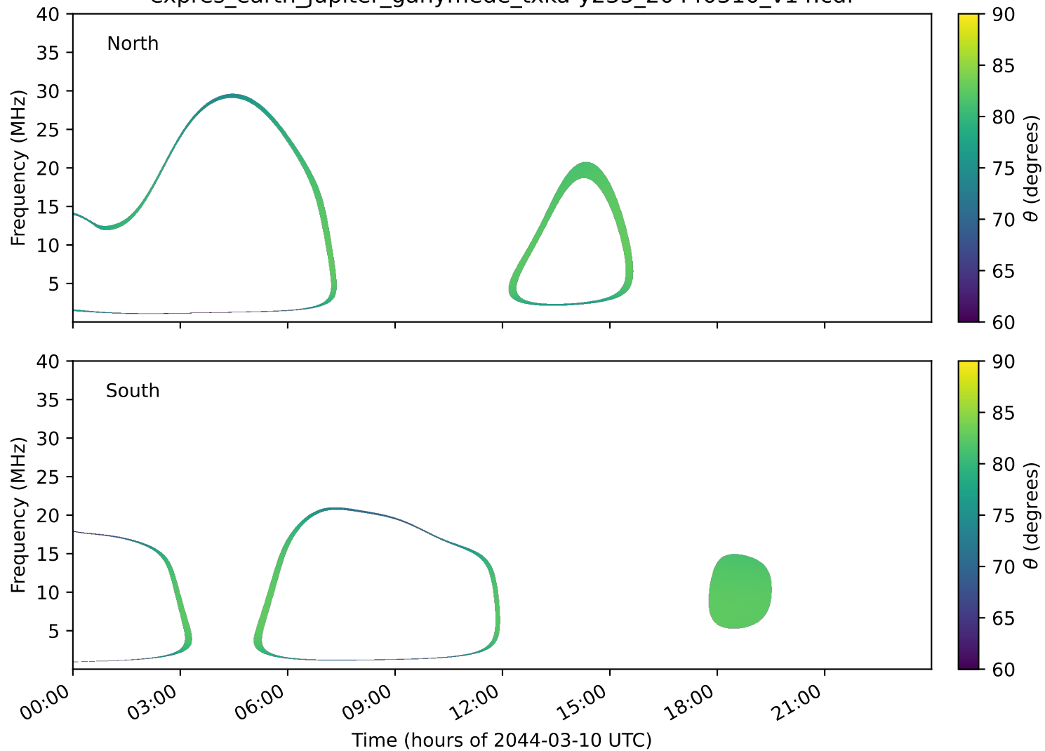
expres_earth_jupiter_ganymede_txka-y235_20440310_v14.cdf
