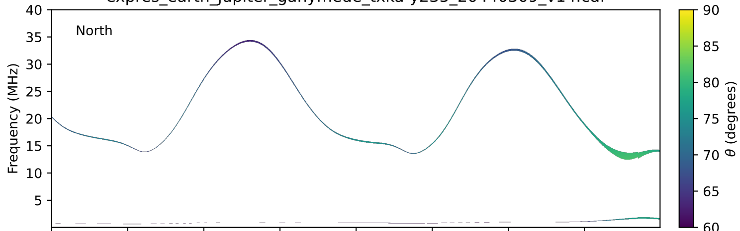
expres_earth_jupiter_ganymede_txka-y235_20440309_v14.cdf
